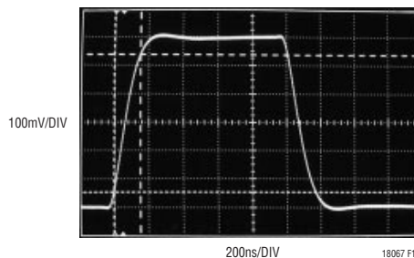
Figure 11. Step Response with R_F = 499k
